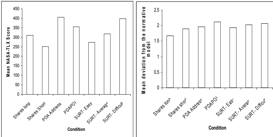
Fig.4. Average NASA-TLX rating and average mean deviation from the normative model by condition
